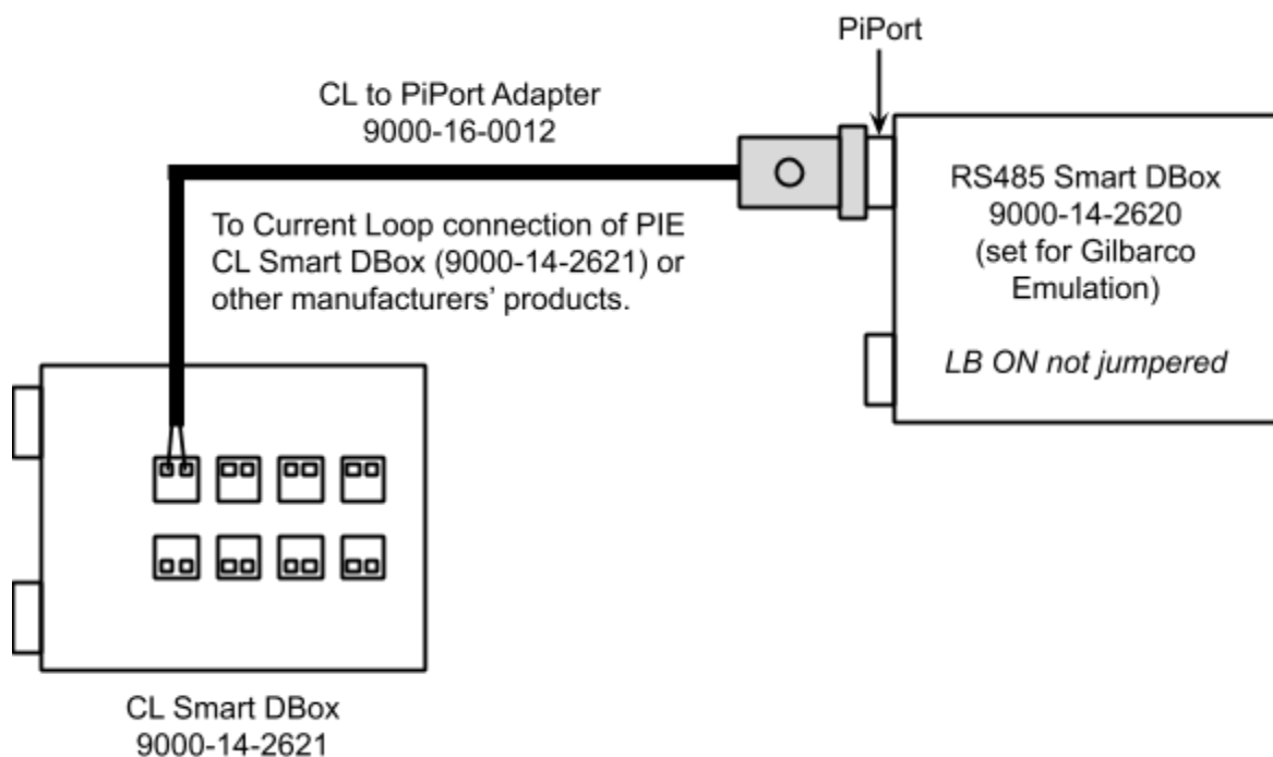
Diagram: CL to PiPort Adapter Connections
